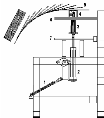
a) Moving a sheet of cardboard
