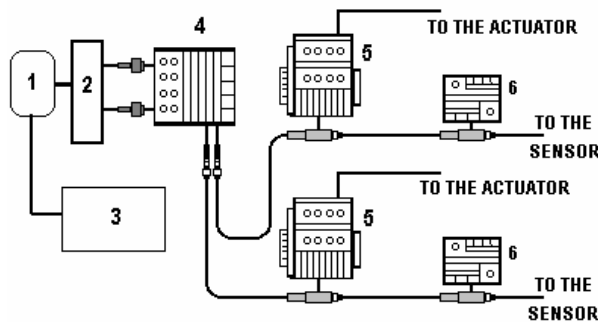
Fig.5 Network arrangement for the control
